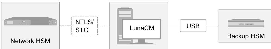
Figure 6: Client-side Local Backup
